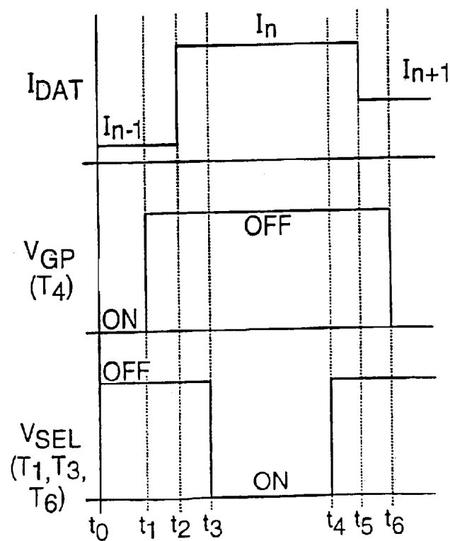
DRIVING WAVEFORM
