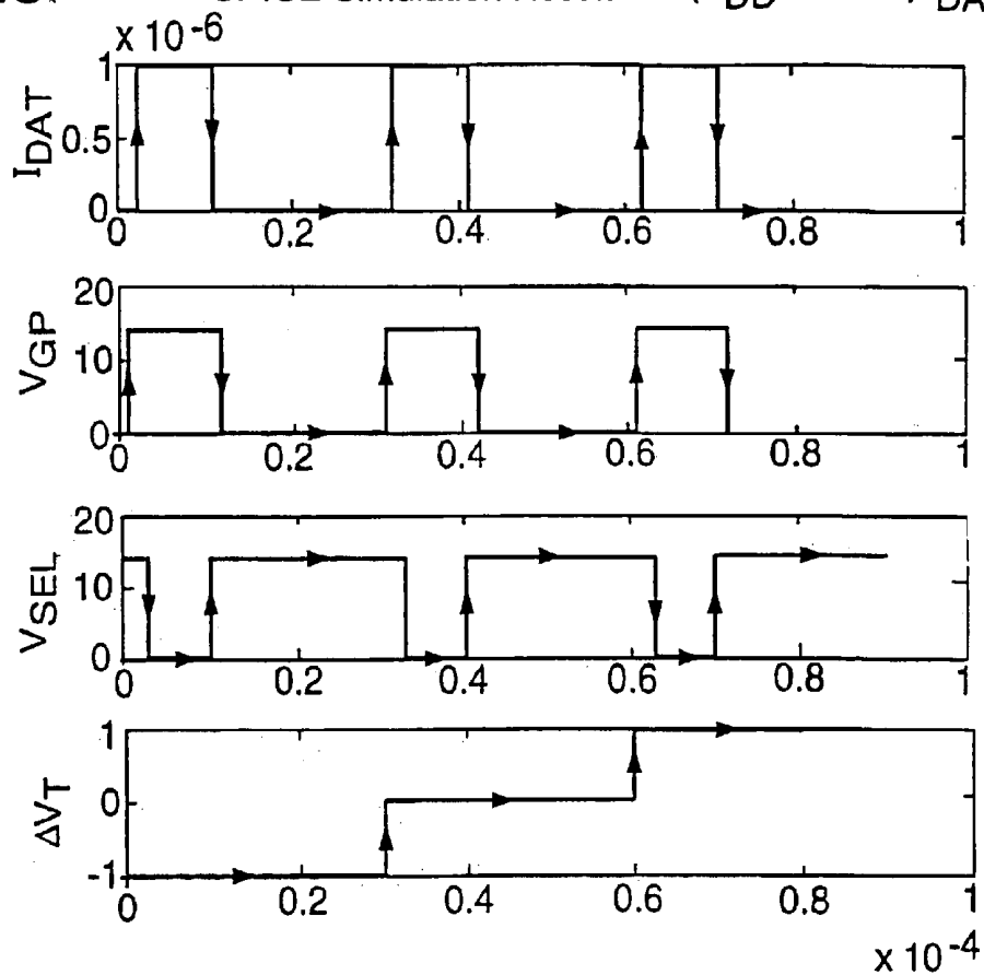
Fig.8. SPICE Simulation Result ( V_{DD}=12.5V , I_{DAT}=\mu A )
